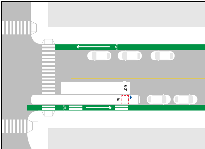
Figure 31 Floating bus stop
