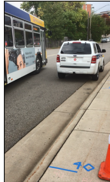
Figure 49 Screenshots showing a 60' bus testing a 40' merge zone a near side stop and a 60' bus testing a 40' merge zone at a far side stop
