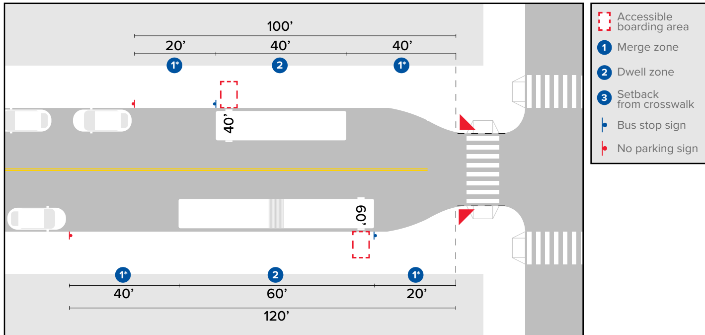
Figure 27 Pull-out bus stop before/after a bumpout, shown for 40 ft. and 60 ft. buses
