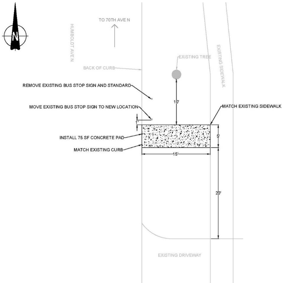
Figure 42 An accessible boarding area (ADA pad) concrete pad installation to connect the sidewalk to the curb over a wide boulevard.
