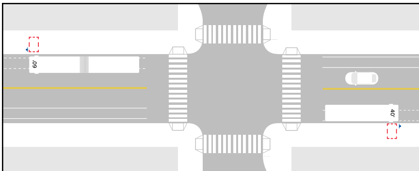
Figure 29 Bus stop and a bus bike mixing zone
