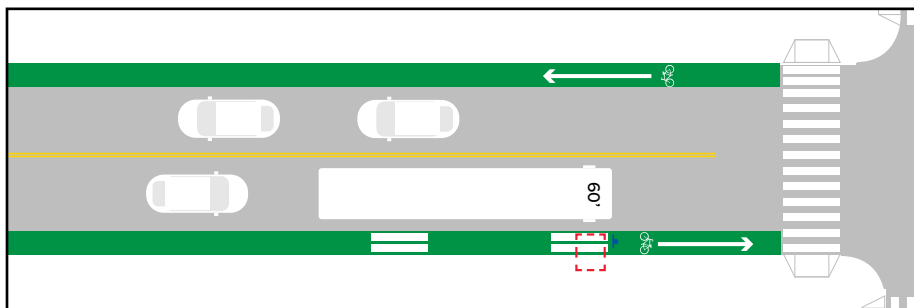
Figure 33 Shared bike-bus stop
