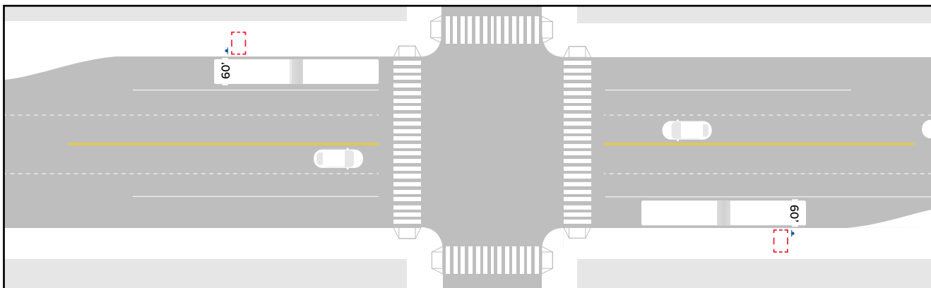
Figure 36 Open bay pull-out stop for high speed roadways
