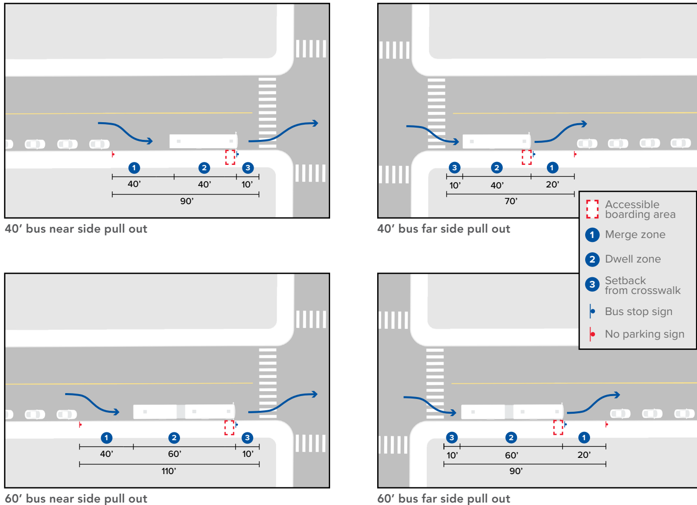
Figure 9 Bus stop zone length required for pull-out stops
