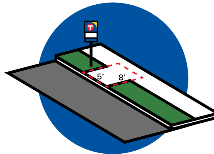
Figure 15 Accessible boarding area (ADA pad)
