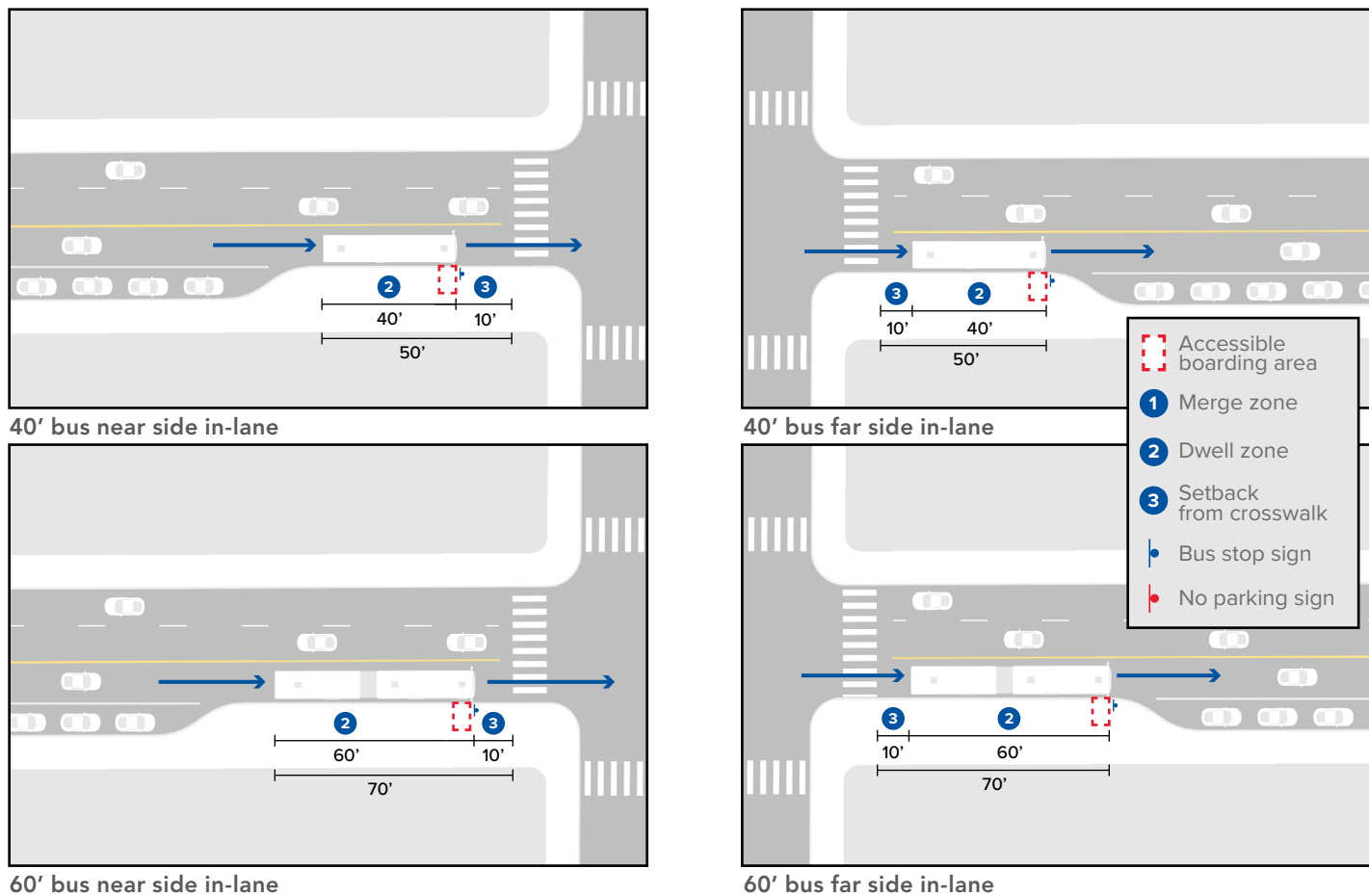
Figure 10 Bus stop zone length required for in-lane stops and stops on a bumpout
