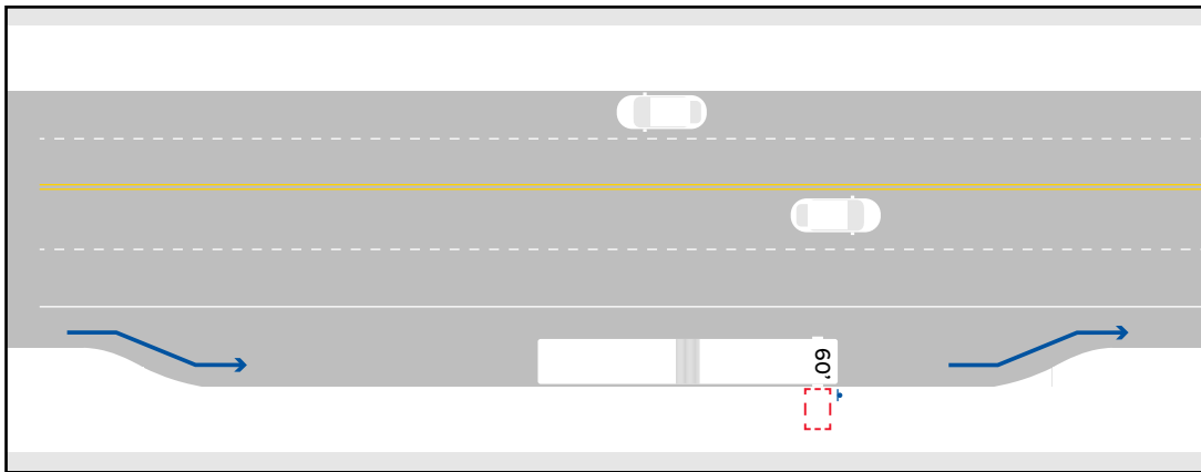
Figure 35 Closed bay pull-out stop for high speed roadways
