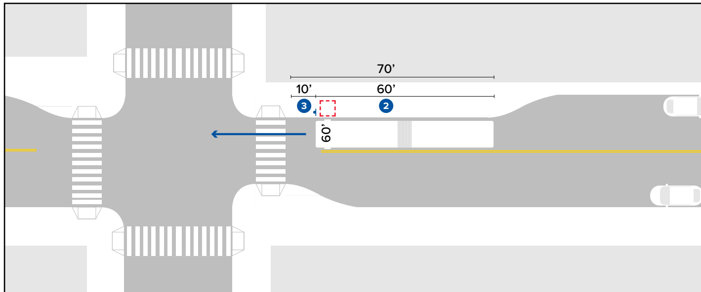
Figure 26 In-lane bus stop sited on a bumpout with appropriate length
