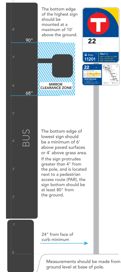
Figure 14 Bus stop sign and bus stop pole installation
