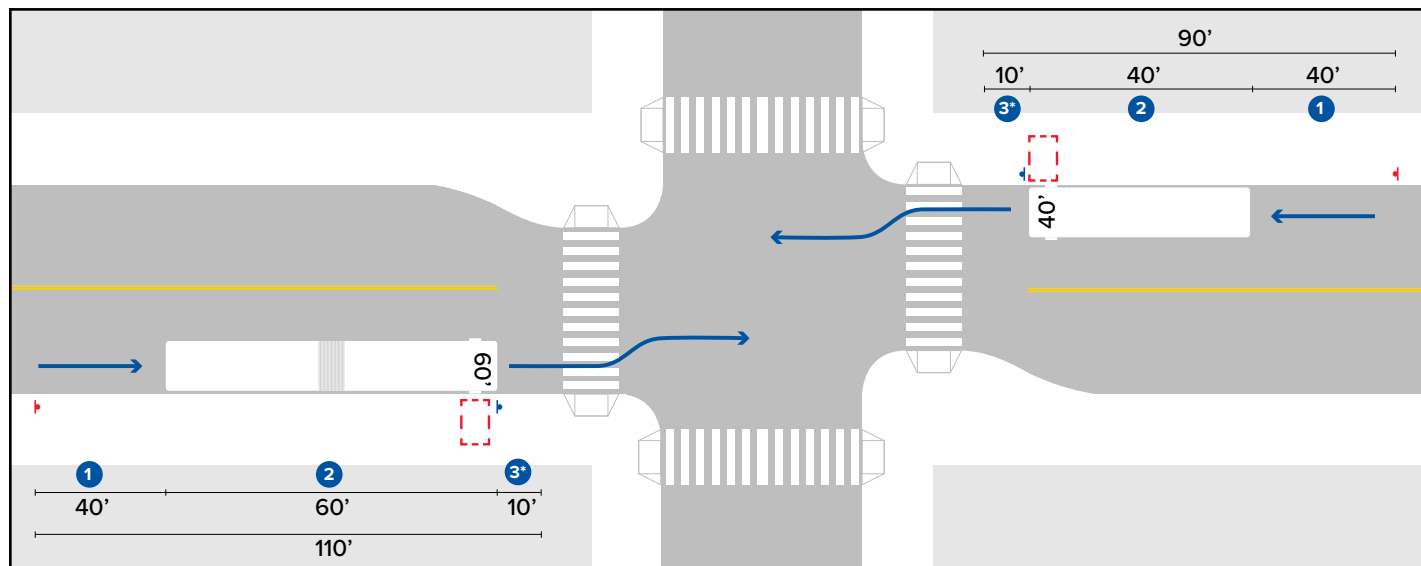
Figure 28 Bumpouts at non-bus stop corners only
