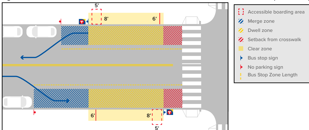
Figure 6 Illustration of the zones in the street and behind the curb for far side and near side pull-out stops
