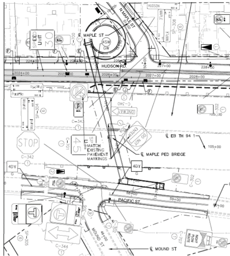
FIGURE 2-13: MAPLE STREET PEDESTRIAN BRIDGE PLAN VIEW – 100% DESIGN
