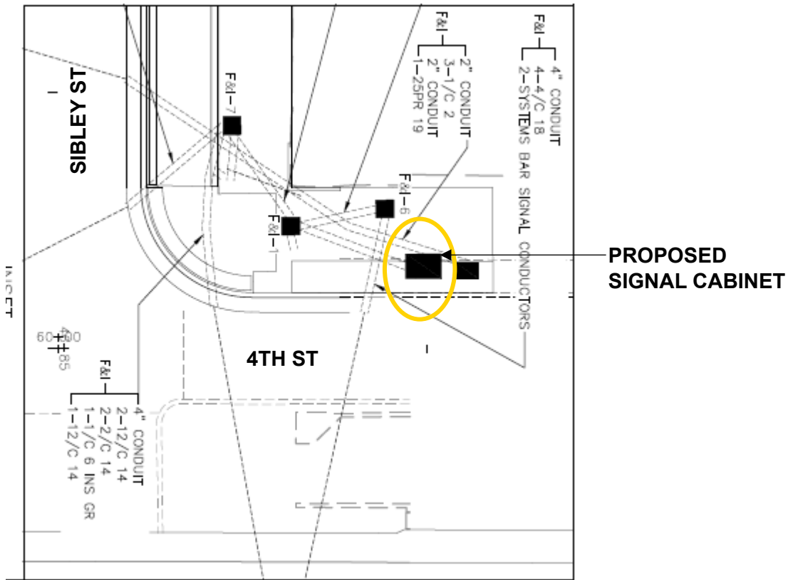
FIGURE 2-8: 4TH STREET AND SIBLEY STREET – 100% DESIGN
