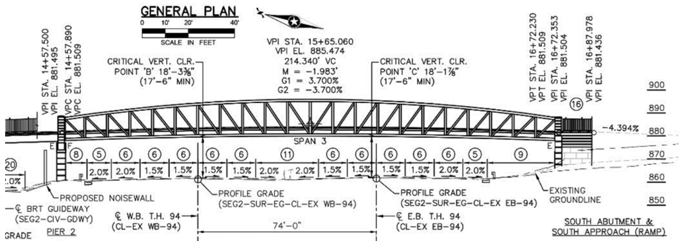
FIGURE 2-12: 90% MAPLE STREET PEDESTRIAN BRIDGE*
