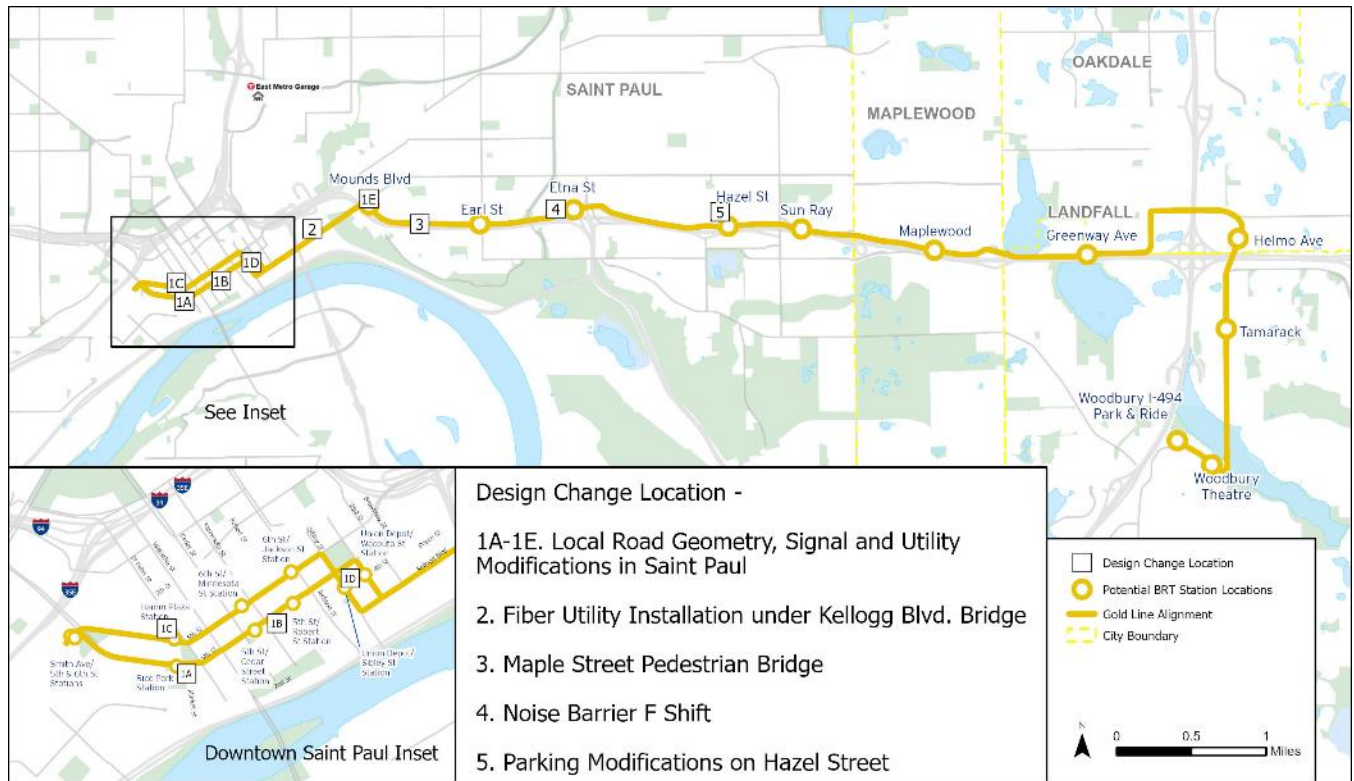
FIGURE 2-1: 100 PERCENT DESIGN CHANGE LOCATIONS
