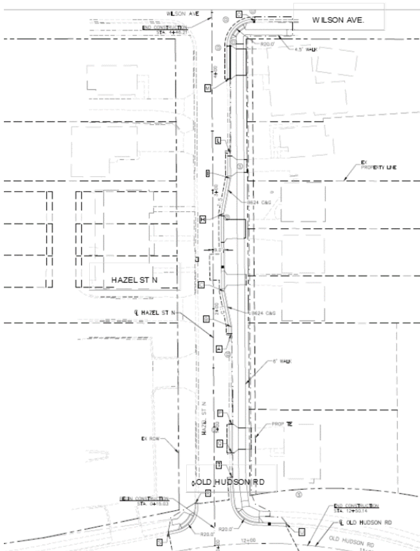
FIGURE 2-14: PARKING MODIFICATIONS ON HAZEL STREET – 100% DESIGN
