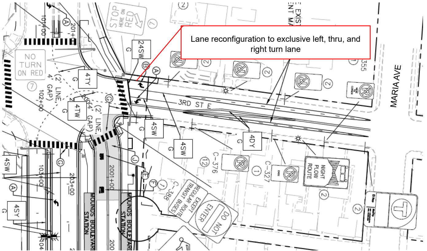
FIGURE 2-9: 3RD STREET INTERSECTION WITH MOUNDS BOULEVARD – 100% DESIGN
