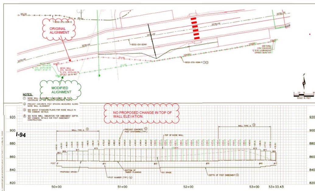
FIGURE 2-16: NOISE BARRIER F – 100% DESIGN
