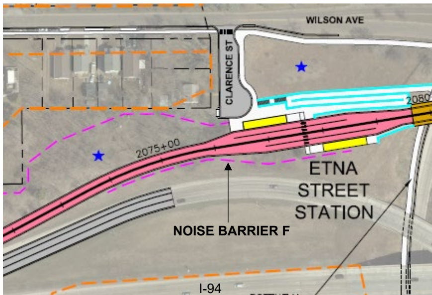
FIGURE 2-16: NOISE BARRIER F – 100% DESIGN
