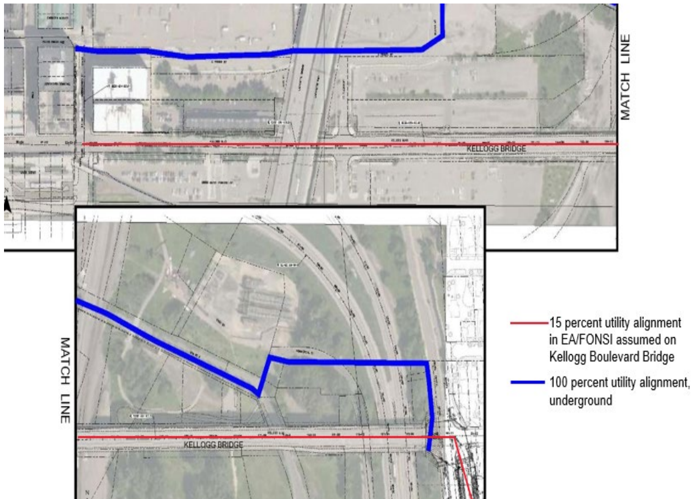
FIGURE 2-10: DOWNTOWN SAINT PAUL FIBER INSTALLATION – 15% DESIGN AND 100% DESIGN
